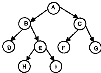
Binary Tree
